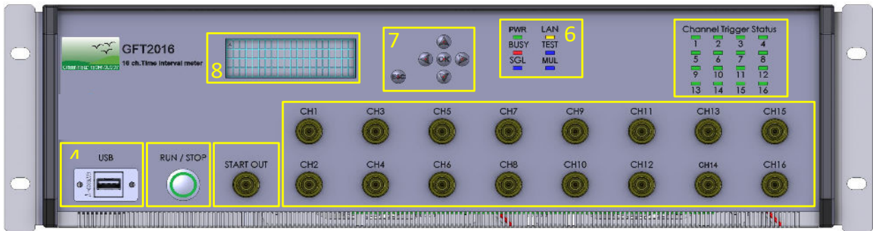
Front panel
