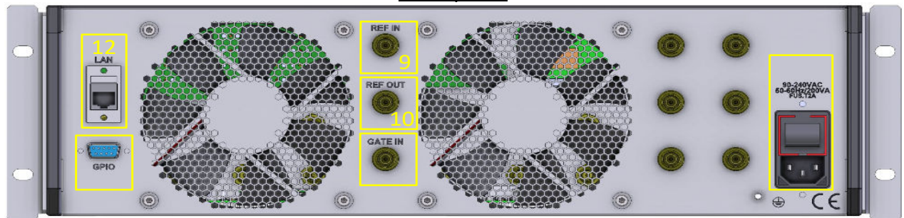
Rear panel
