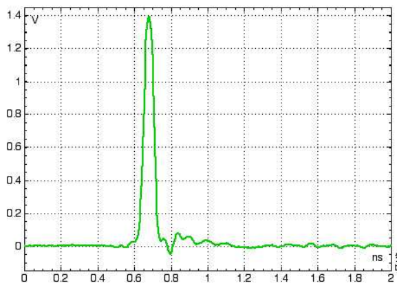
50 PS IMPULSE RESPONSE (with a 20 ps Armexel 4015B PPL pulser)
